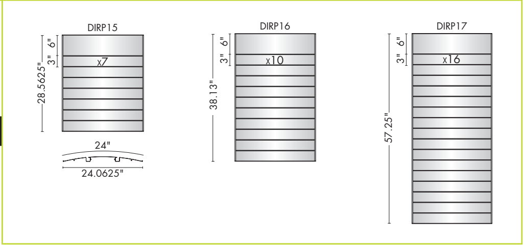
All length measurements apply to the extrusion only and exclude the end caps.
